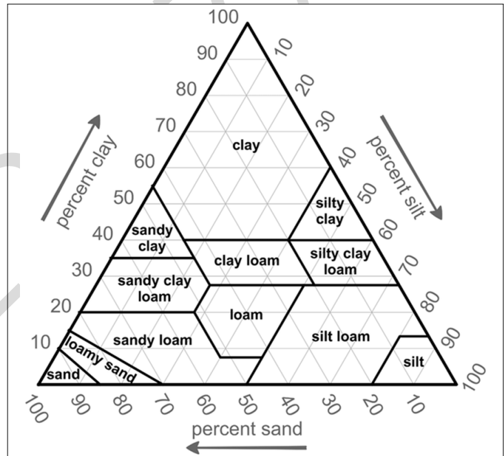
Soil Texture Triangle
